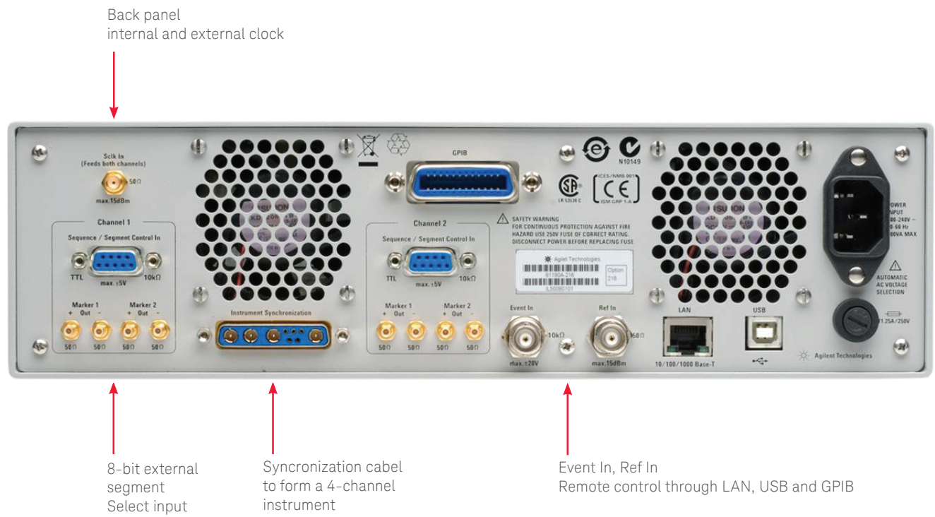
Figure 3. Back panel
